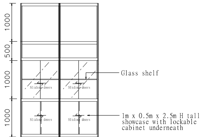
VIEW A
