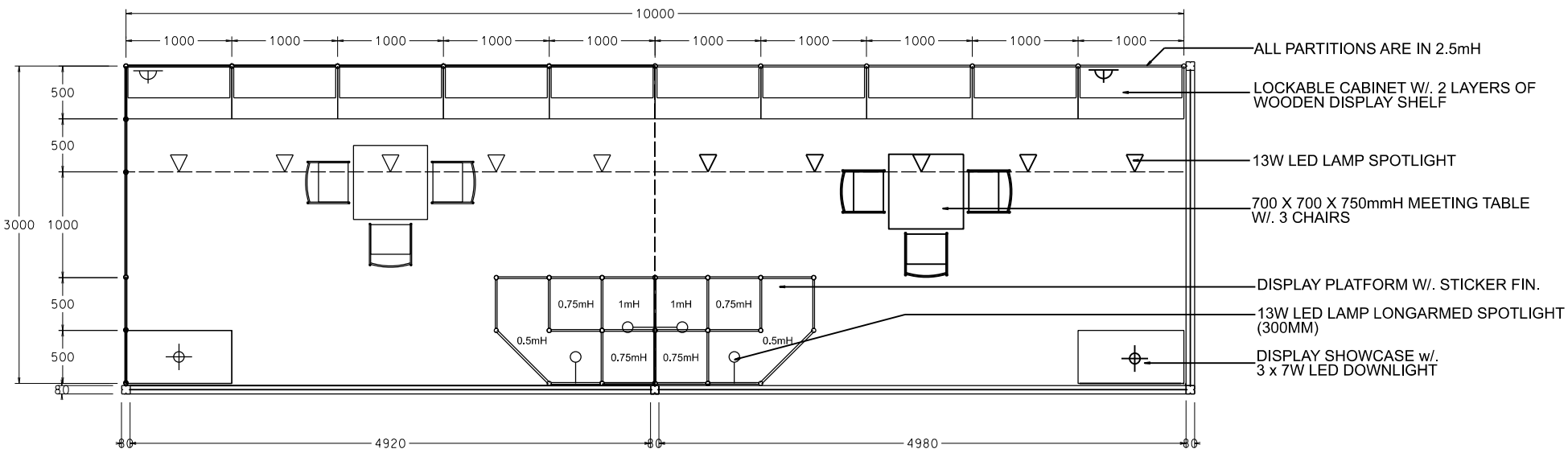
PLAN
