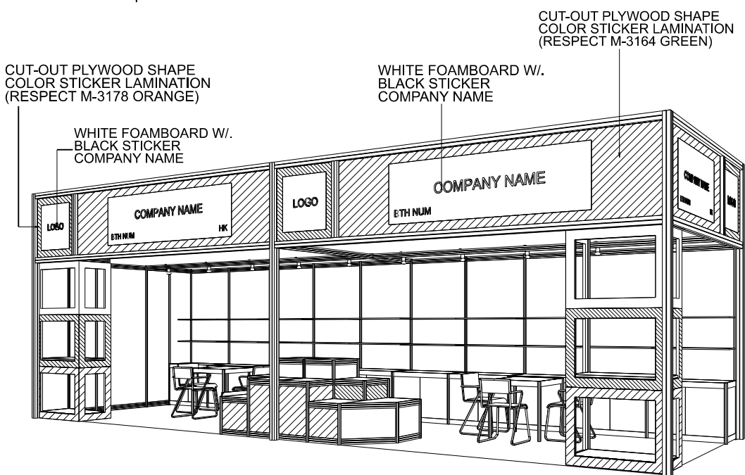
PERSPECTIVE
